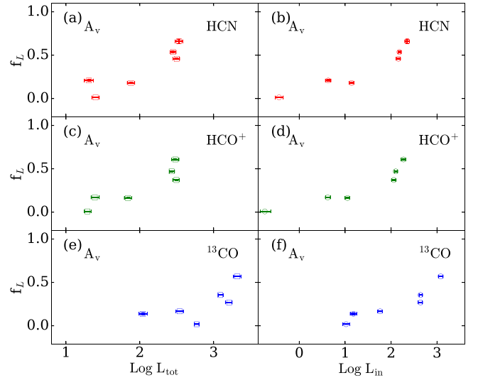
Figure 4. The fraction of line luminosity arising above A_V \geq 8 mag plotted vs. line luminosity. HCN is plotted in the top row, HCO + in the middle row, and 13 CO in the bottom row. The total line luminosities ( \text{Log } L_{\text{tot}} ) are on the left and luminosity from the “in” region ( \text{Log } L_{\text{in}} ) on the right.
