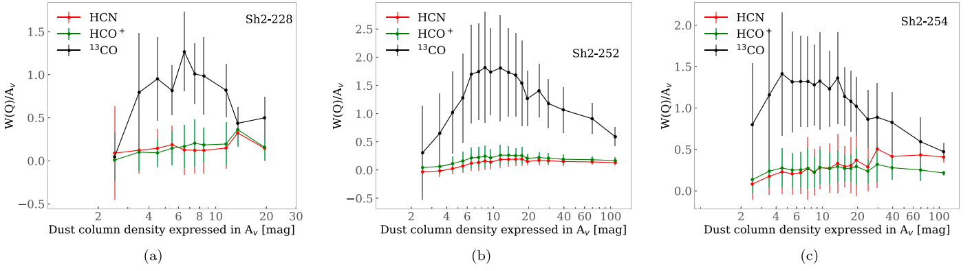
Figure 6. Line-to-mass ratio is plotted against A_V based on Herschel dust column density for the regions (a) S228, (b) S252, and (c) S254.
