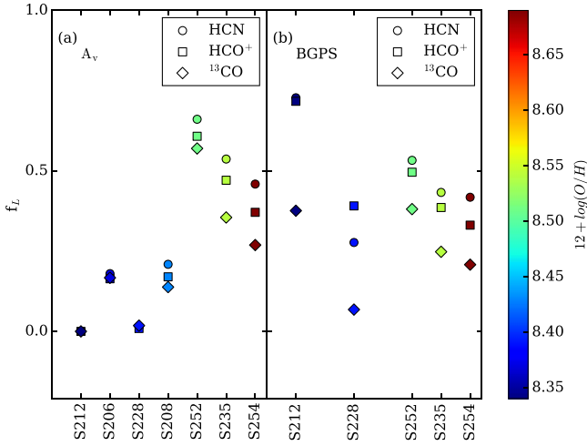
Figure 3. The fraction of luminosity ( f_L ) within the “in” region is plotted for each tracer vs. clouds. The f_L in the left panel is obtained from the A_V \geq 8 mag region, and in the right panel f_L is from the BGPS mask region. The targets are organized with increasing metallicity. Different symbols are used to separate the different tracers. Different colors indicate the metallicity of each source.
