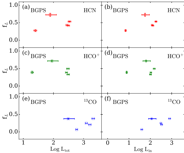
Figure 5. The fraction of line luminosity arising from the BGPS mask region plotted vs. line luminosity. HCN is plotted in the top row, HCO + in the middle row, and 13 CO in the bottom row. The total line luminosities (Log L_{\text{tot}} ) are on the left and luminosity from the "in" region (Log L_{\text{in}} ) on the right.
