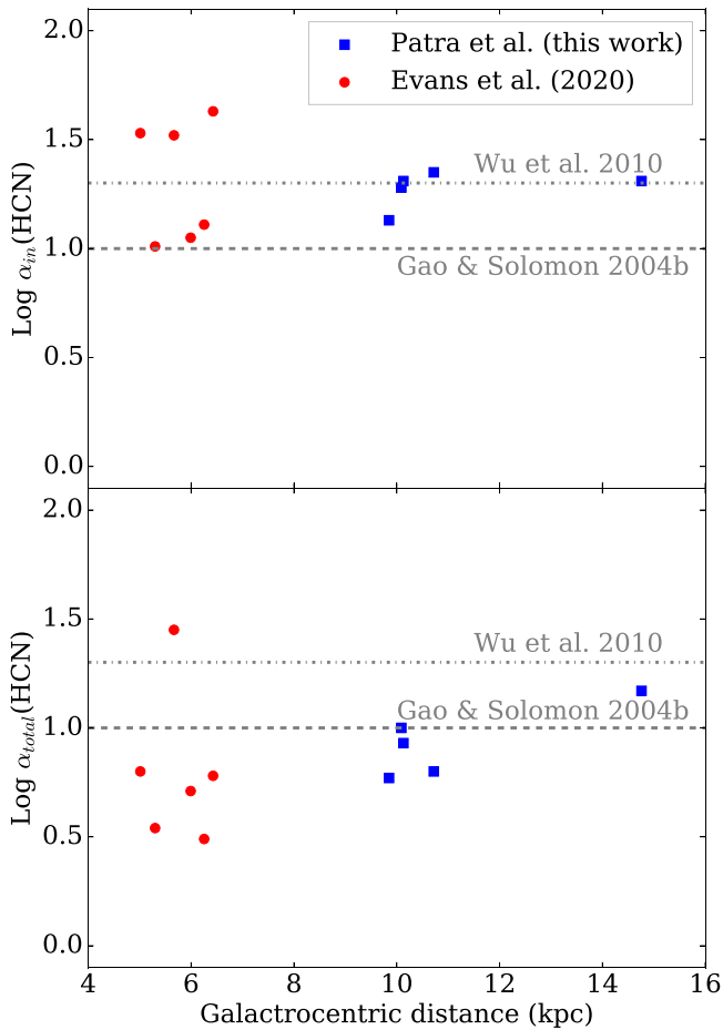
Figure 8. Variation of conversions factors \text{Log } \alpha_{in}(\text{HCN}) and \text{Log } \alpha_{tot}(\text{HCN}) for inner and outer Galaxy targets with Galactocentric distance ( R_G ).
